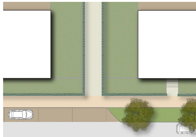
Figure 94: Illustrative diagram showing an indicative layout of on-street inset parking.
